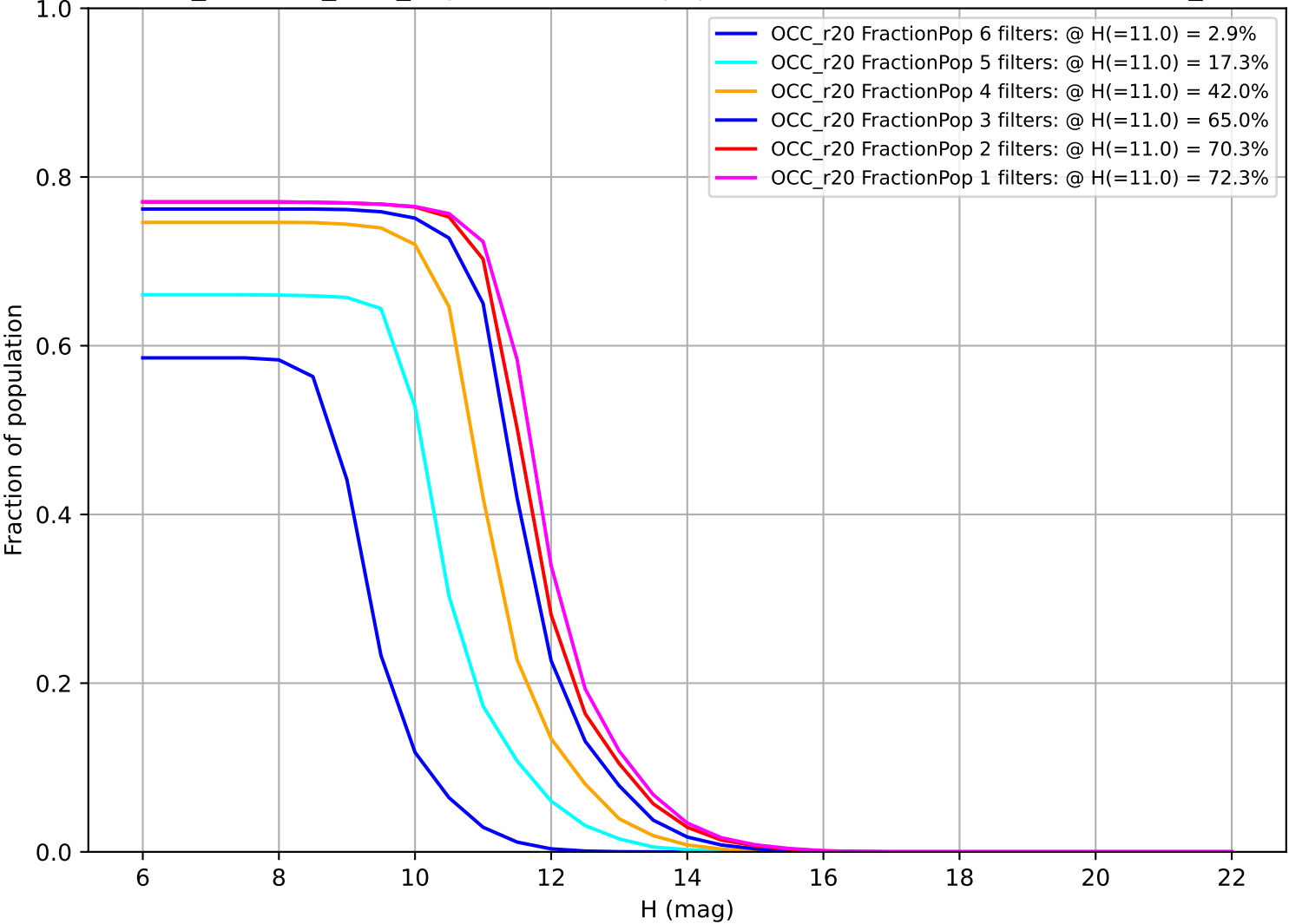
retro_baseline_v2.0_10yrs: Fraction of population with colors in X filters OCC_r20
