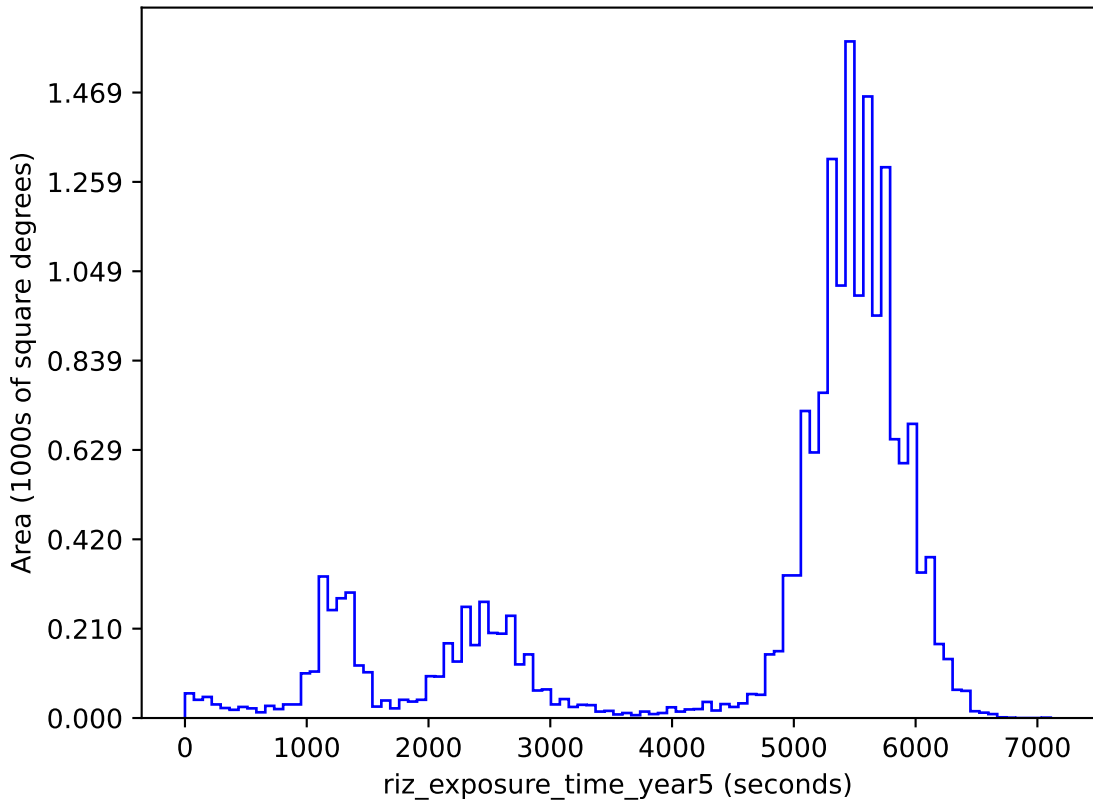
retro_baseline_v2.0_10yrs gri band non-DD: riz_exposure_time_year5
