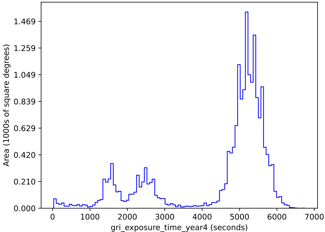
retro_baseline_v2.0_10yrs gri band non-DD: gri_exposure_time_year4
