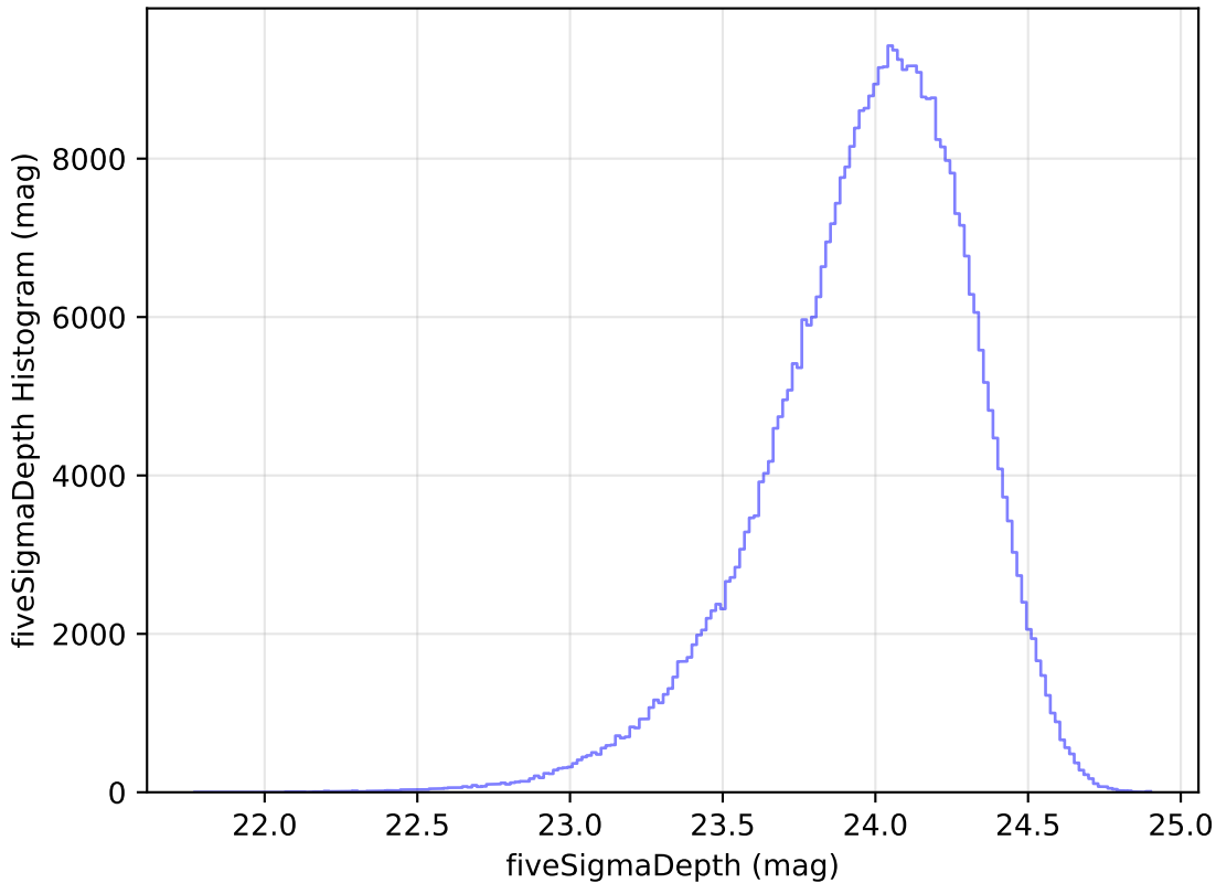
retro_baseline_v2.0_10yrs r: fiveSigmaDepth Histogram
