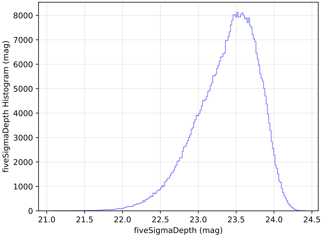
retro_baseline_v2.0_10yrs i: fiveSigmaDepth Histogram
