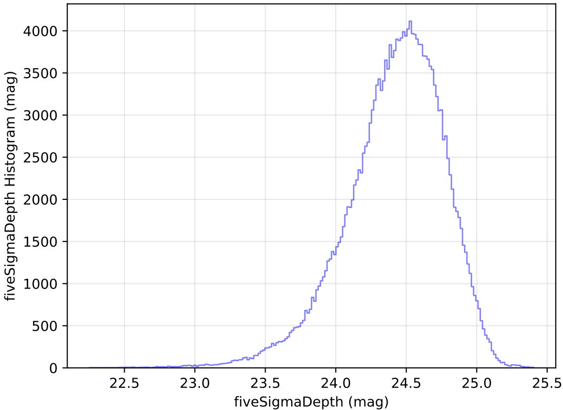
retro_baseline_v2.0_10yrs g: fiveSigmaDepth Histogram
