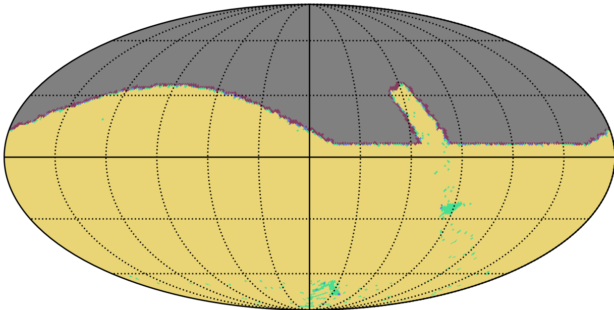
retro_baseline_v2.0_10yrs z band: YearCoverage night
