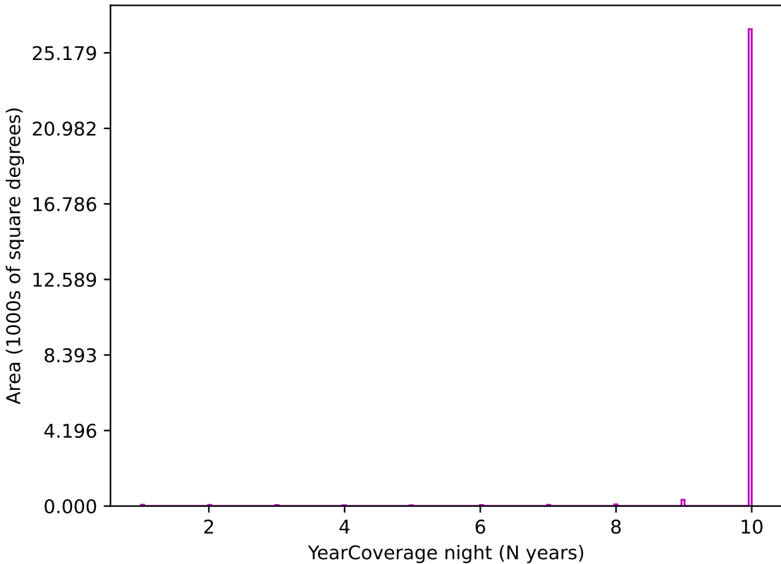
retro_baseline_v2.0_10yrs z band: YearCoverage night
