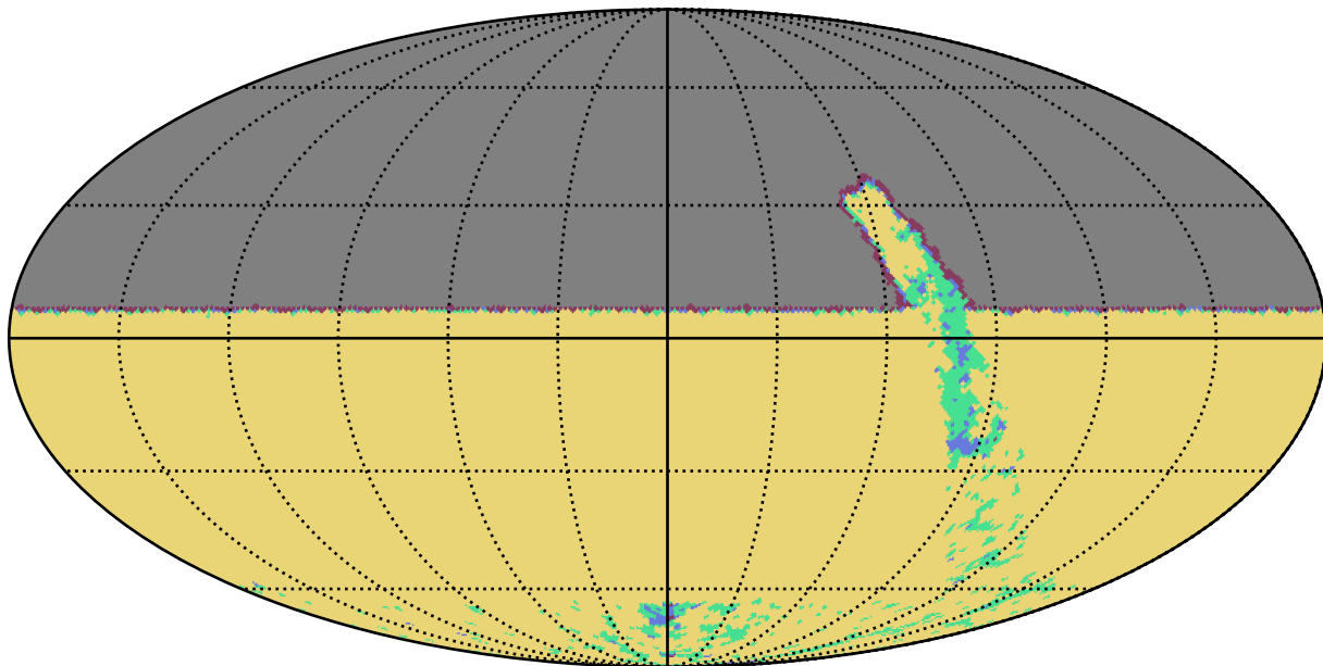
retro_baseline_v2.0_10yrs y band: YearCoverage night
