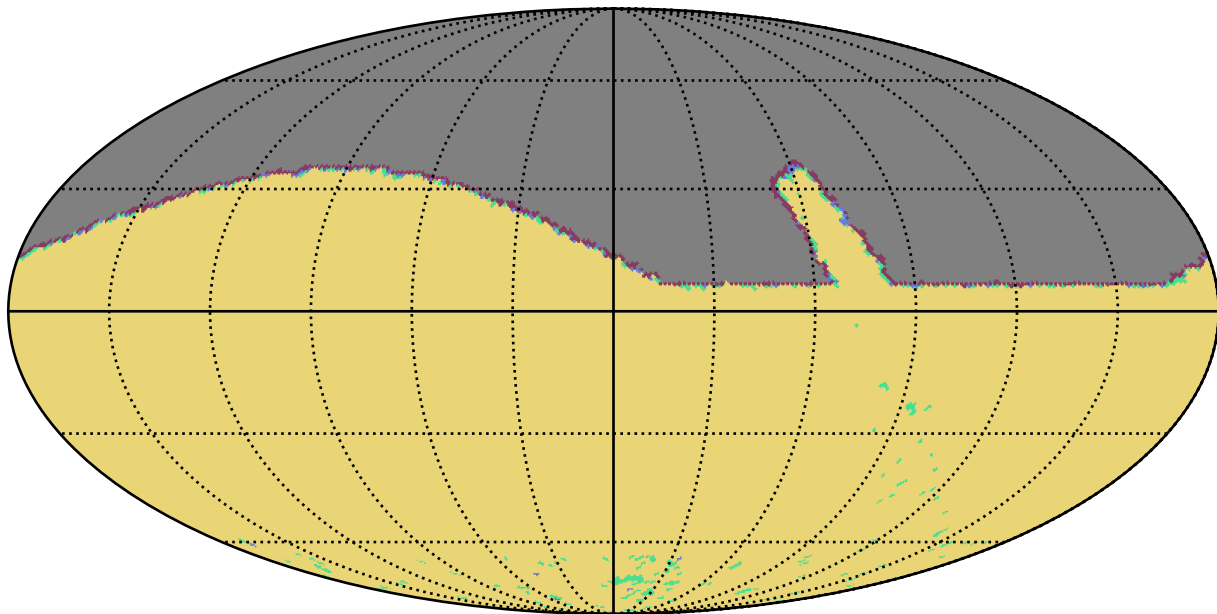
retro_baseline_v2.0_10yrs r band: YearCoverage night
