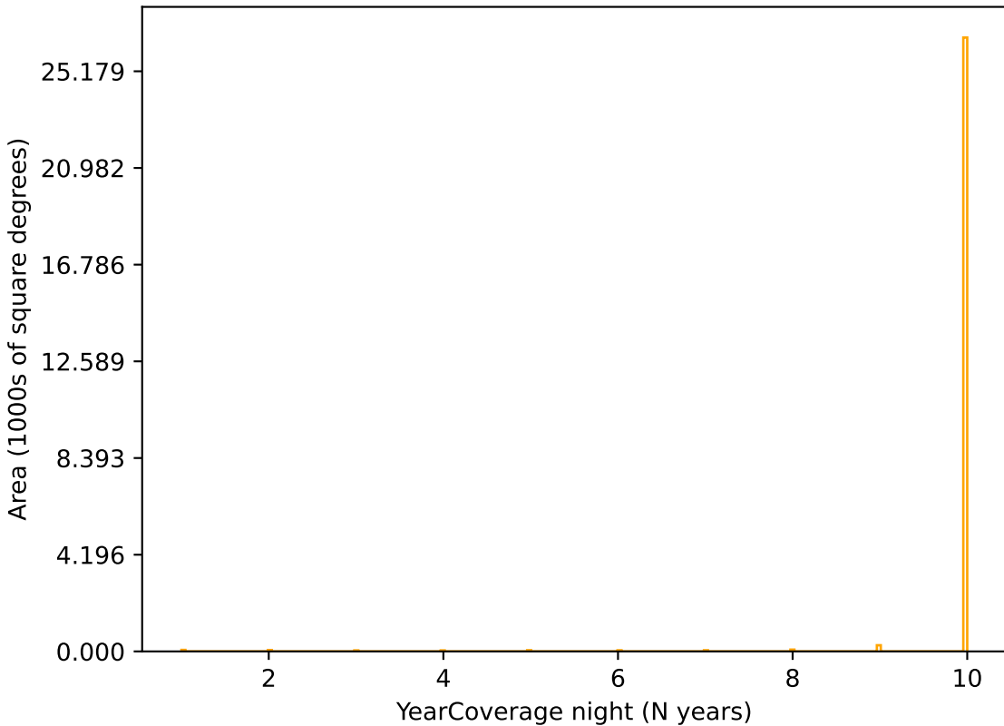
retro_baseline_v2.0_10yrs r band: YearCoverage night
