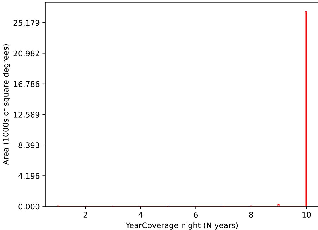
retro_baseline_v2.0_10yrs i band: YearCoverage night
