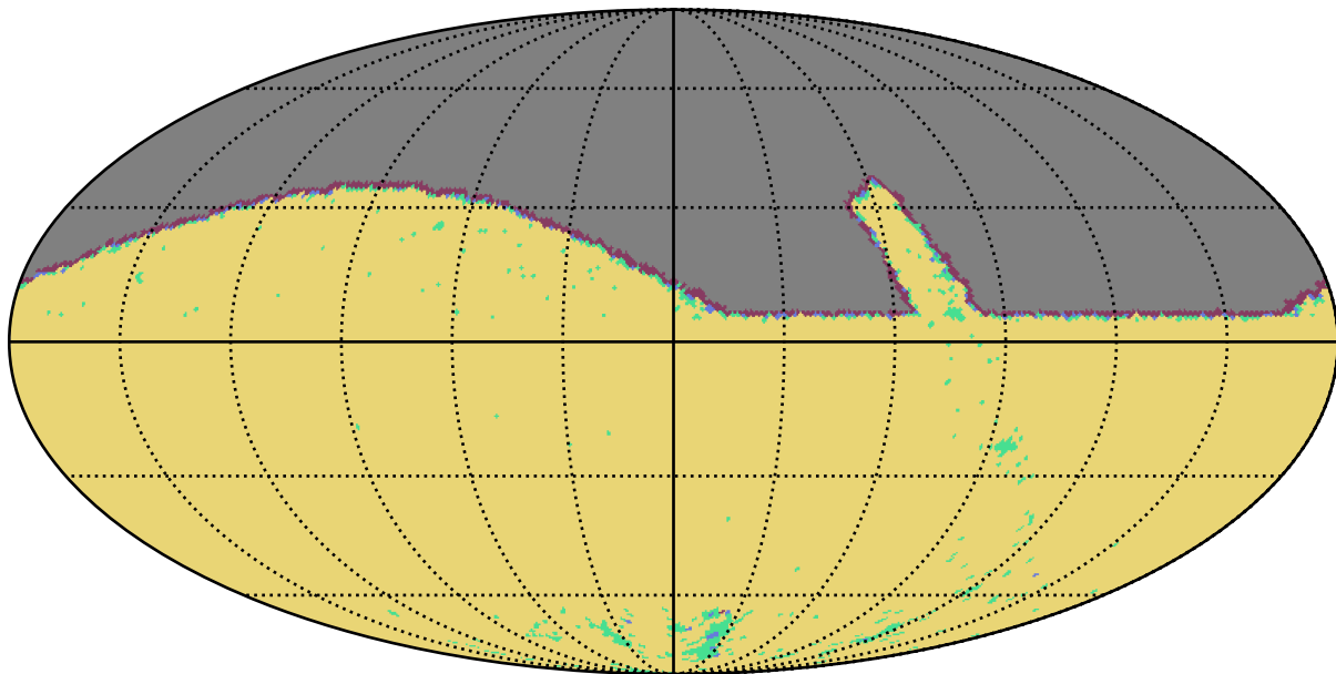
retro_baseline_v2.0_10yrs g band: YearCoverage night
