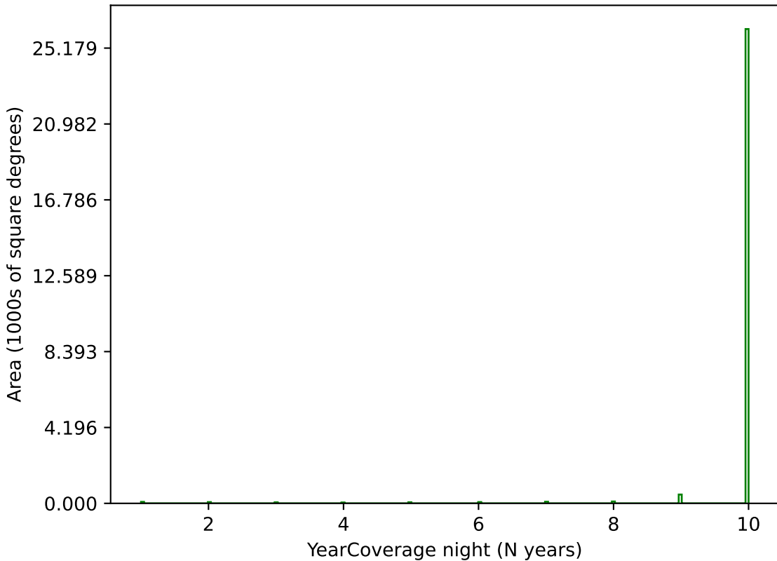
retro_baseline_v2.0_10yrs g band: YearCoverage night
