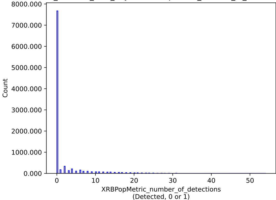
retro_baseline_v2.0_10yrs : XRBPoMetric_number_of_detections
