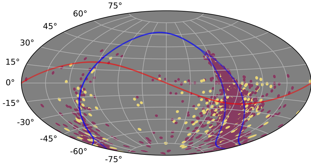
retro_baseline_v2.0_10yrs : XRBPopMetric_early_detect
