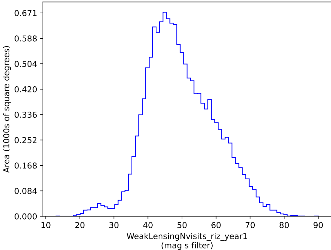
retro_baseline_v2.0_10yrs gri band non-DD: WeakLensingNvisits_riz_year1
