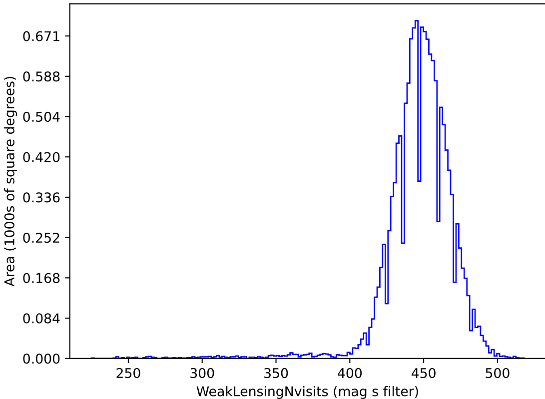
retro_baseline_v2.0_10yrs gri band non-DD: WeakLensingNvisits
