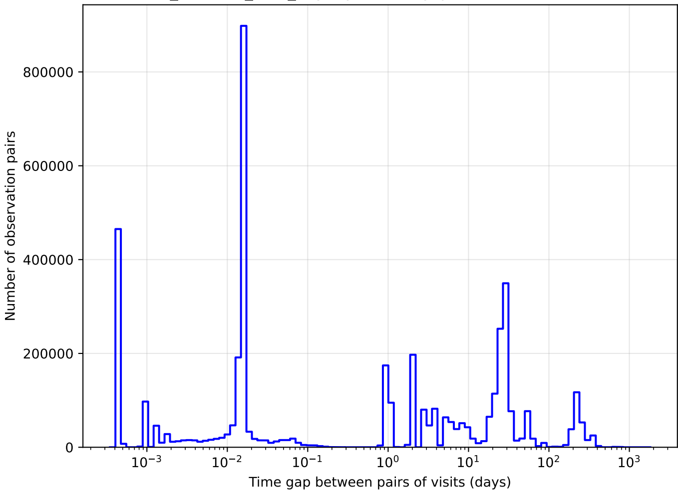
retro_baseline_v2.0_10yrs y band: Tgaps observationStartMJD
