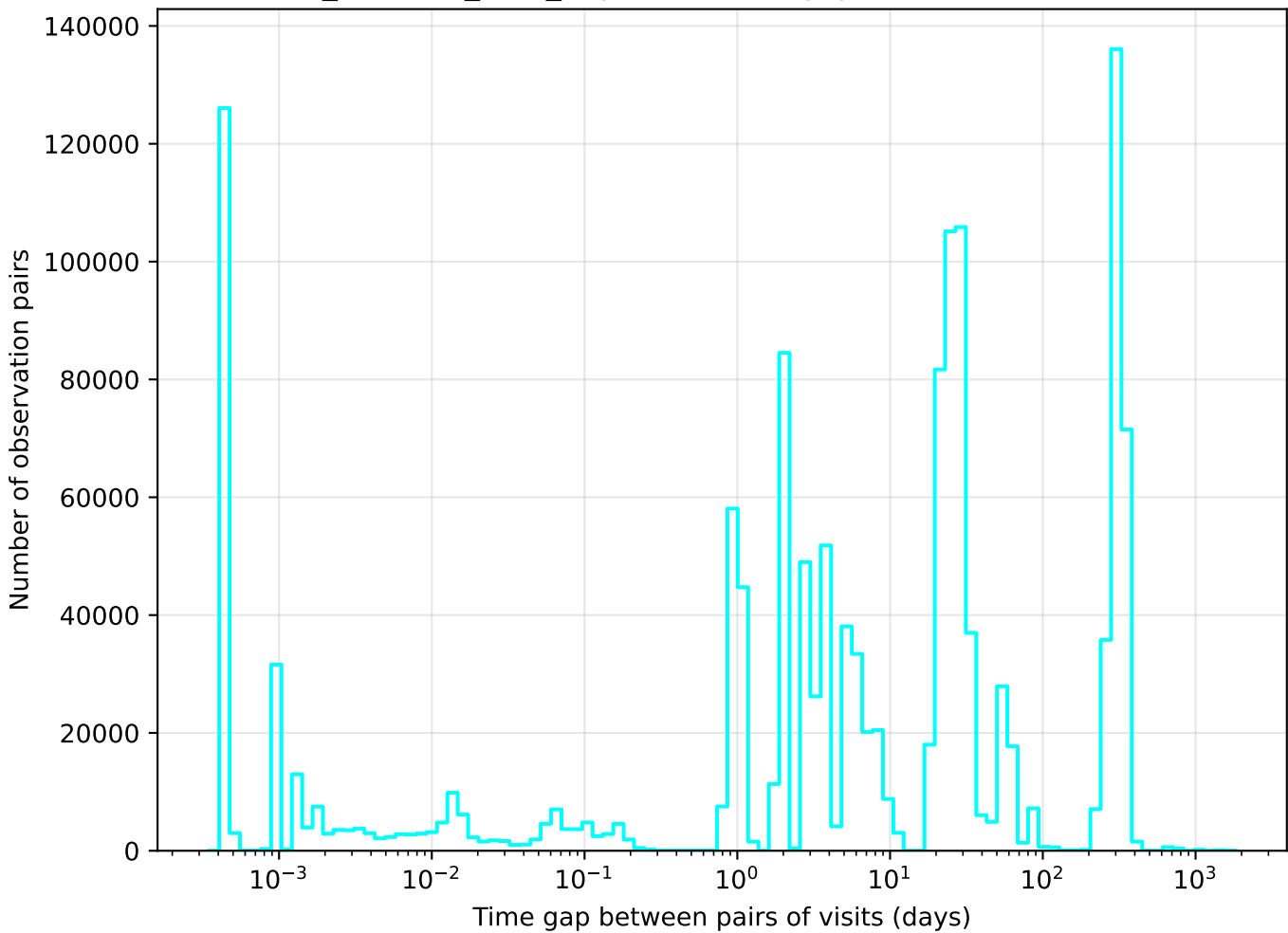
retro_baseline_v2.0_10yrs u band: Tgaps observationStartMJD
