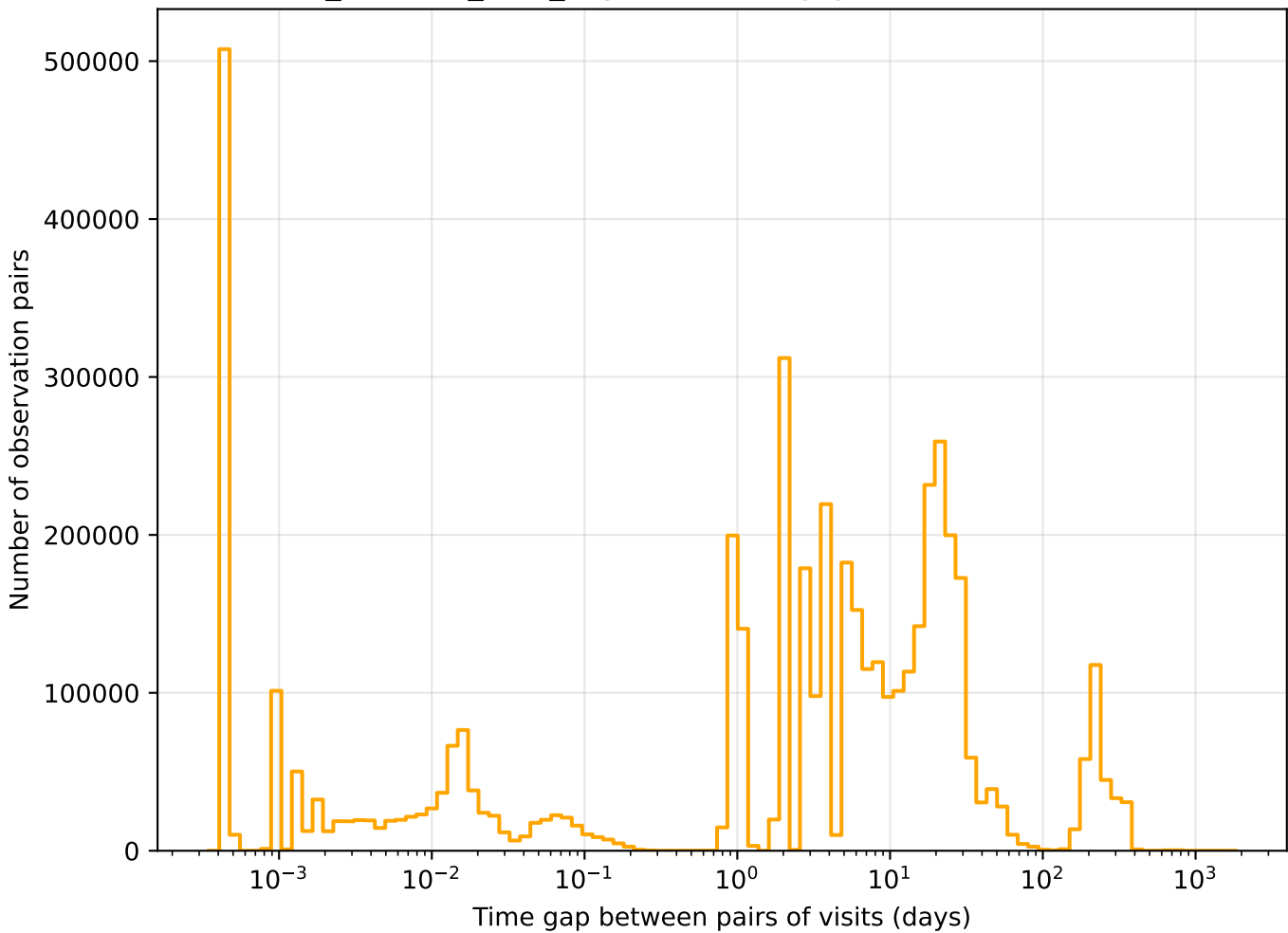
retro_baseline_v2.0_10yrs r band: Tgaps observationStartMJD
