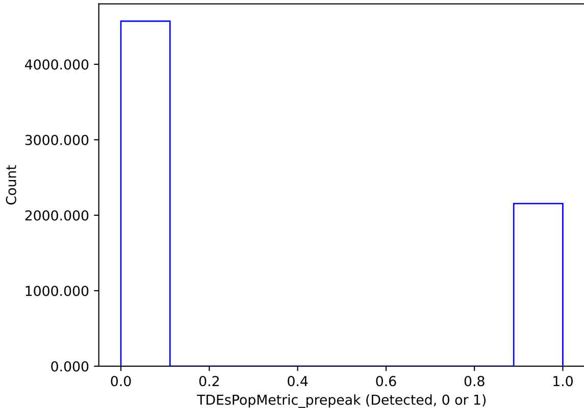
retro_baseline_v2.0_10yrs : TDEsPopMetric_prepeak
