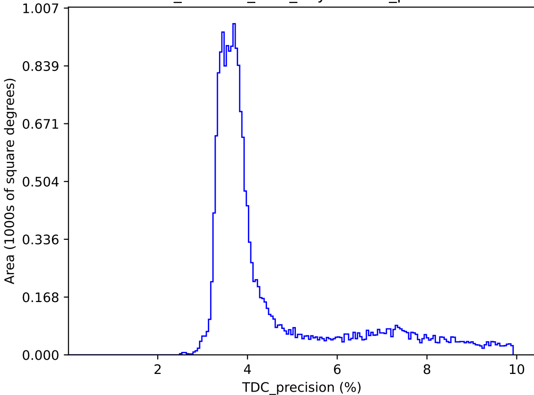
retro_baseline_v2.0_10yrs : TDC_precision
