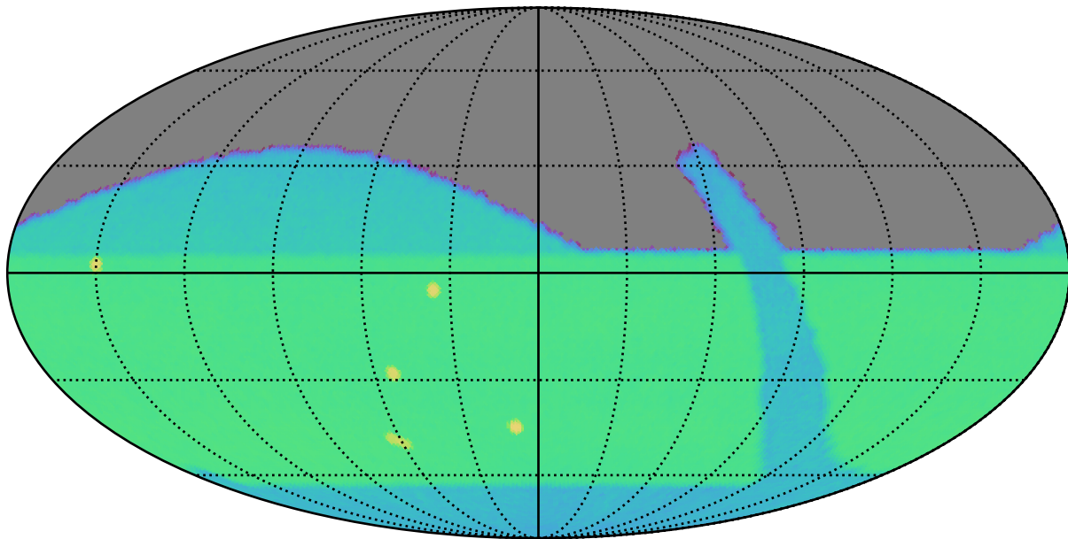
retro_baseline_v2.0_10yrs z: SurfaceBrightLimit
