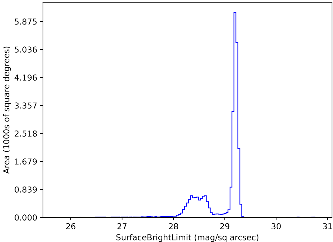
retro_baseline_v2.0_10yrs z: SurfaceBrightLimit
