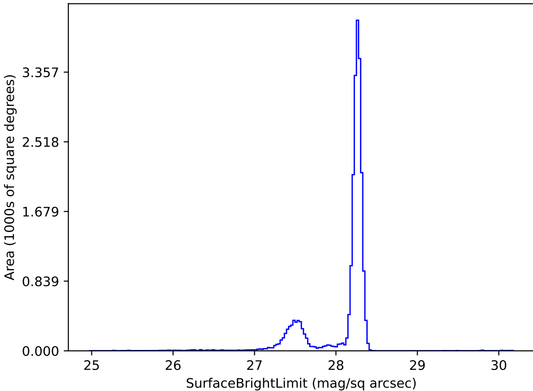
retro_baseline_v2.0_10yrs y: SurfaceBrightLimit
