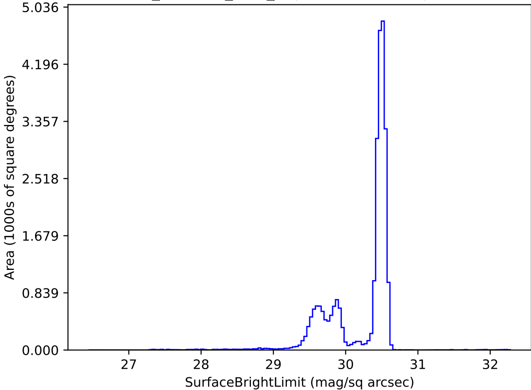
retro_baseline_v2.0_10yrs r: SurfaceBrightLimit
