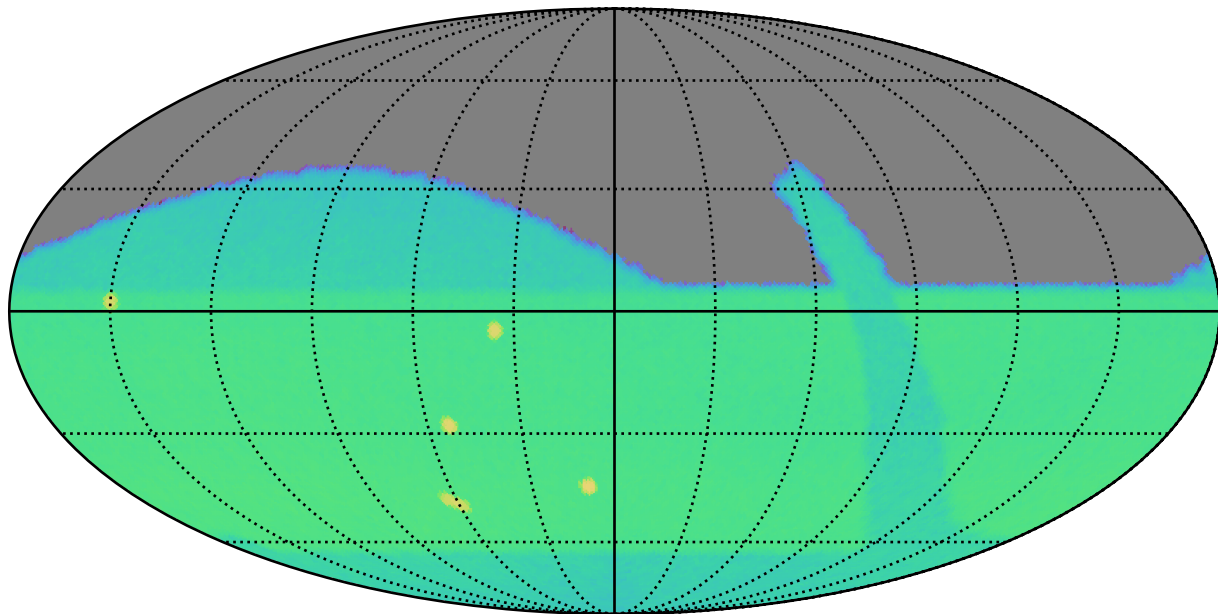
retro_baseline_v2.0_10yrs g: SurfaceBrightLimit
