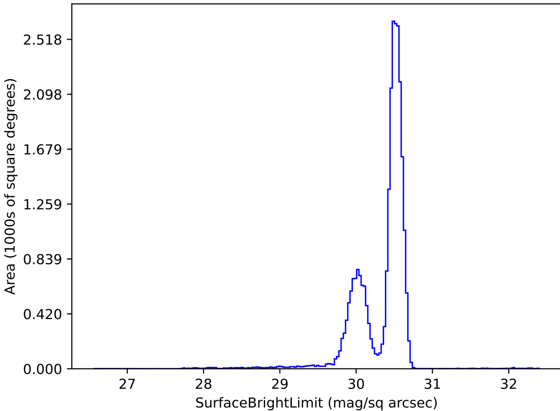
retro_baseline_v2.0_10yrs g: SurfaceBrightLimit
