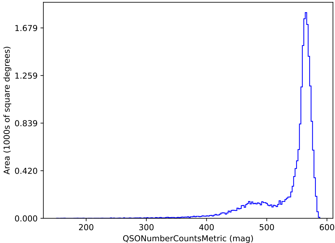
retro_baseline_v2.0_10yrs y band and non-DD: QSONumberCountsMetric
