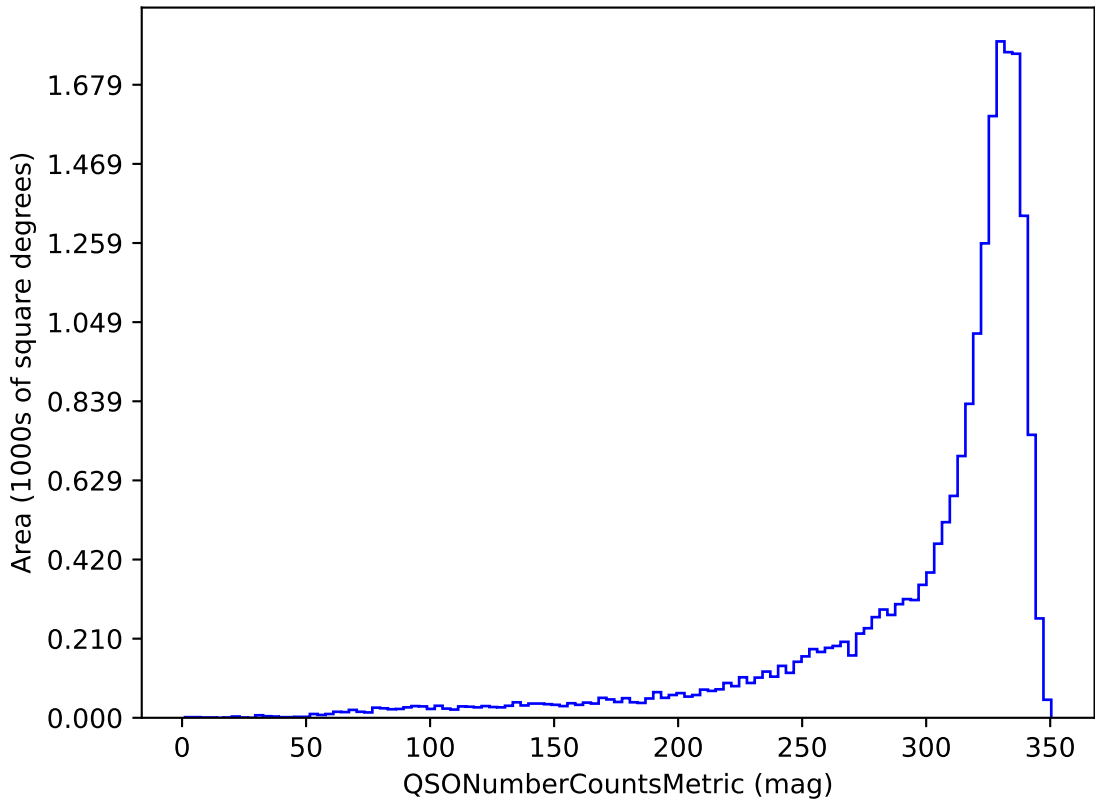
retro_baseline_v2.0_10yrs u band and non-DD: QSONumberCountsMetric
