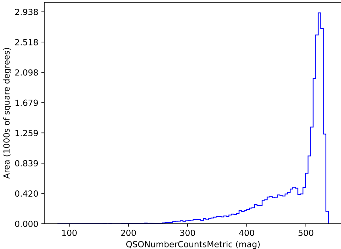
retro_baseline_v2.0_10yrs r band and non-DD: QSONumberCountsMetric
