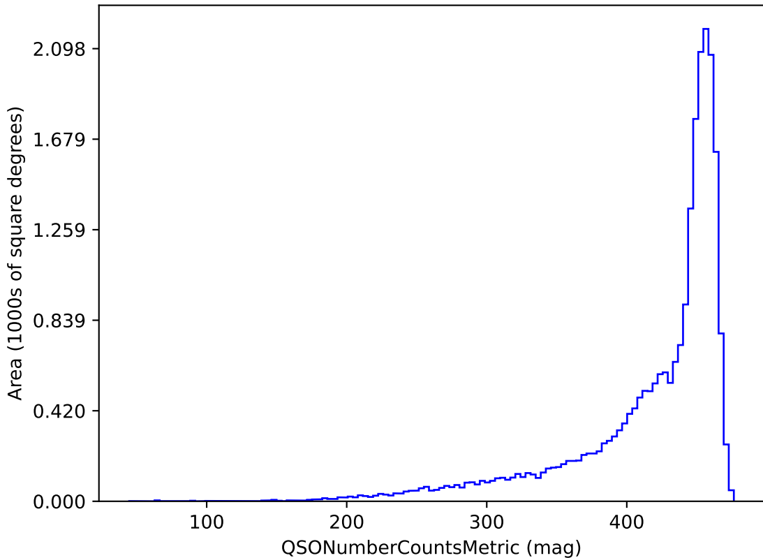
retro_baseline_v2.0_10yrs g band and non-DD: QSONumberCountsMetric
