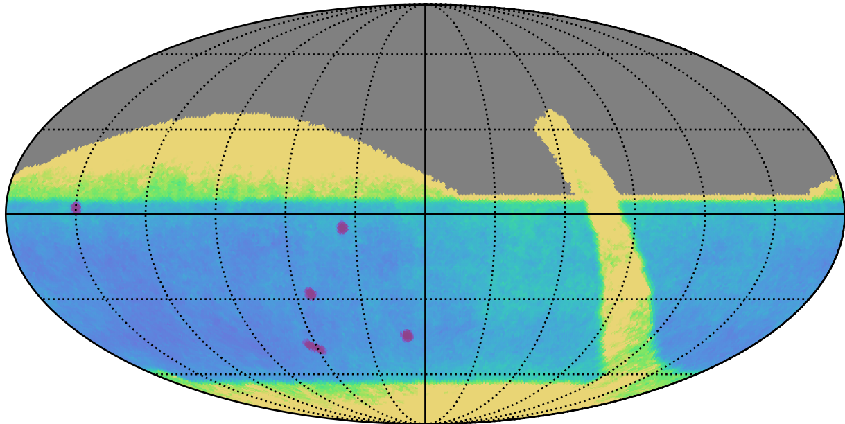
retro_baseline_v2.0_10yrs : Proper Motion Uncert @ 24.0
