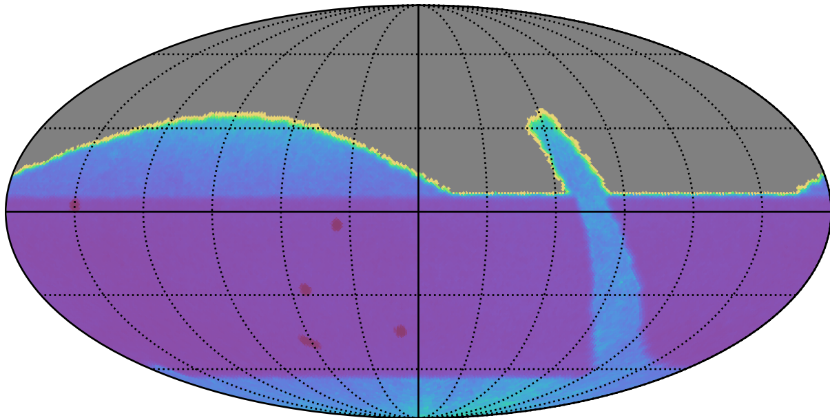
retro_baseline_v2.0_10yrs : Proper Motion Uncert @ 20.5
