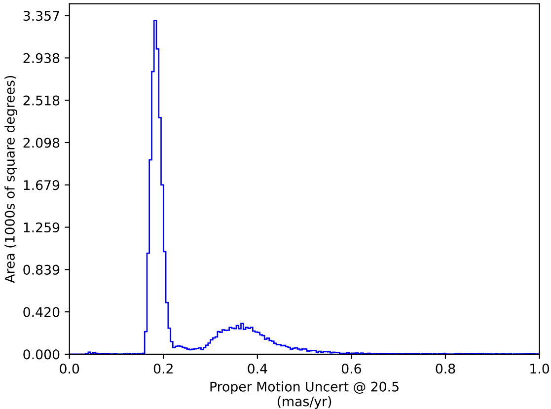
retro_baseline_v2.0_10yrs : Proper Motion Uncert @ 20.5
