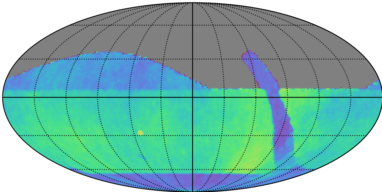
retro_baseline_v2.0_10yrs : Parallax Coverage @ 22.4
