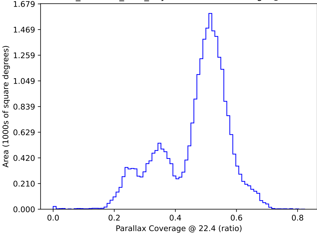
retro_baseline_v2.0_10yrs : Parallax Coverage @ 22.4
