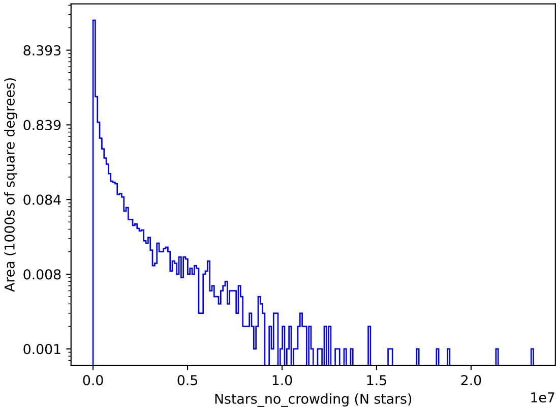
retro_baseline_v2.0_10yrs z: Nstars_no_crowding
