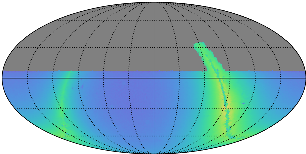
retro_baseline_v2.0_10yrs y: Nstars_no_crowding
