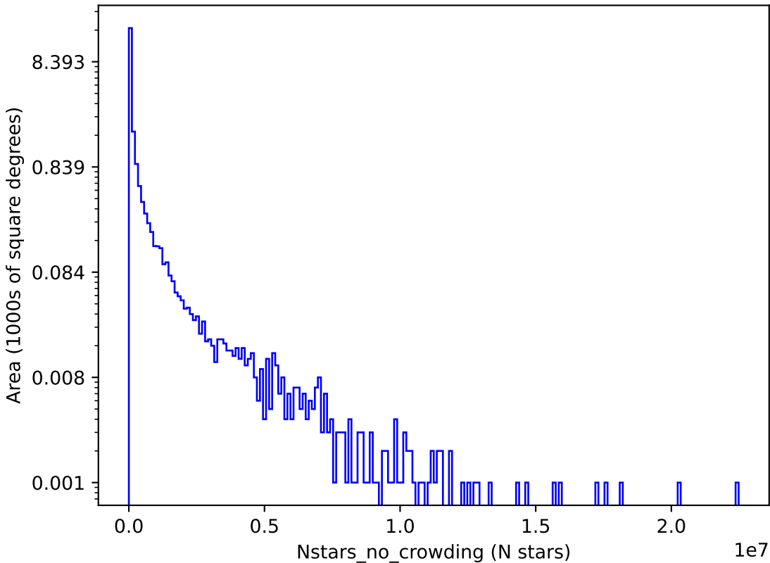
retro_baseline_v2.0_10yrs y: Nstars_no_crowding
