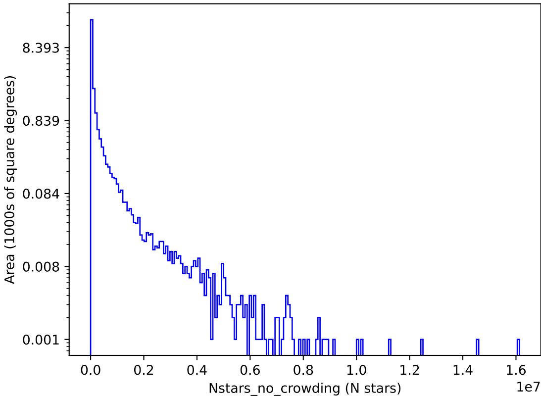
retro_baseline_v2.0_10yrs r: Nstars_no_crowding
