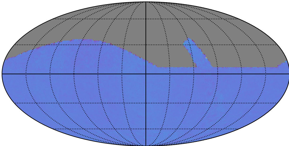
retro_baseline_v2.0_10yrs : Normalized Proper Motion Uncert @ 20.5
