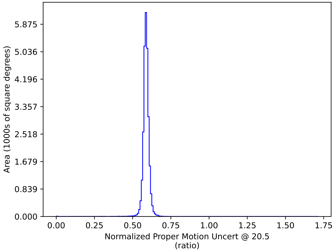
retro_baseline_v2.0_10yrs : Normalized Proper Motion Uncert @ 20.5
