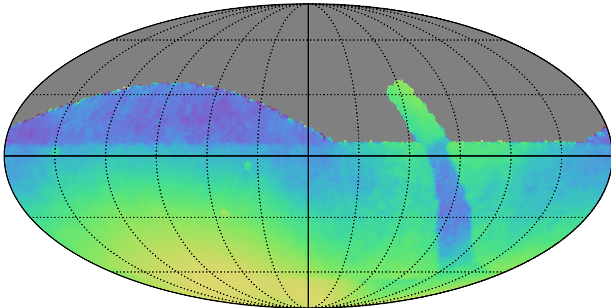
retro_baseline_v2.0_10yrs : Normalized Parallax Uncert @ 24.0
