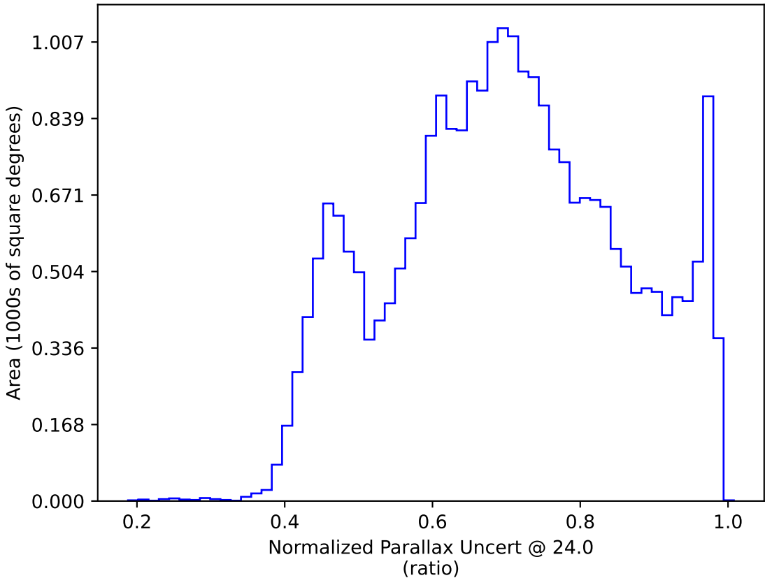
retro_baseline_v2.0_10yrs : Normalized Parallax Uncert @ 24.0
