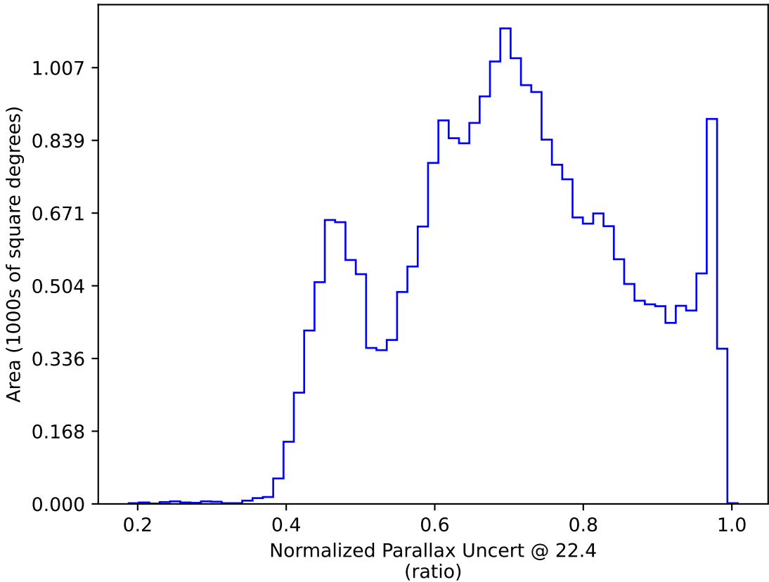
retro_baseline_v2.0_10yrs : Normalized Parallax Uncert @ 22.4
