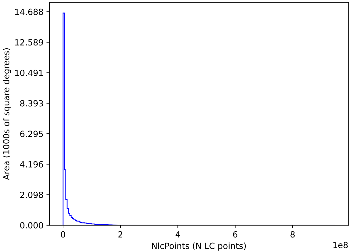
retro_baseline_v2.0_10yrs : NlcPoints
