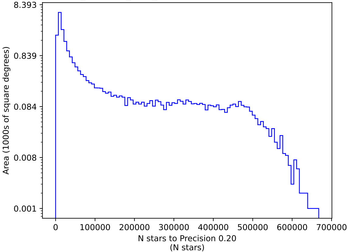
retro_baseline_v2.0_10yrs y: N stars to Precision 0.20
