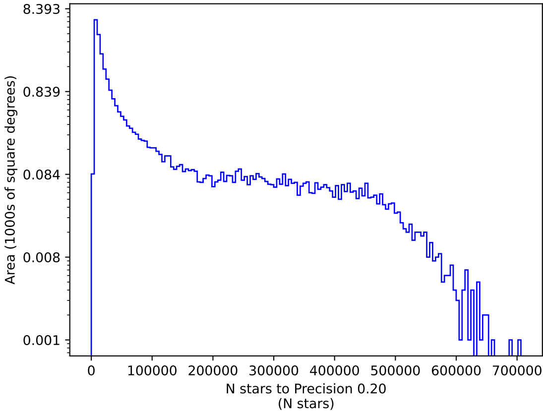
retro_baseline_v2.0_10yrs r: N stars to Precision 0.20
